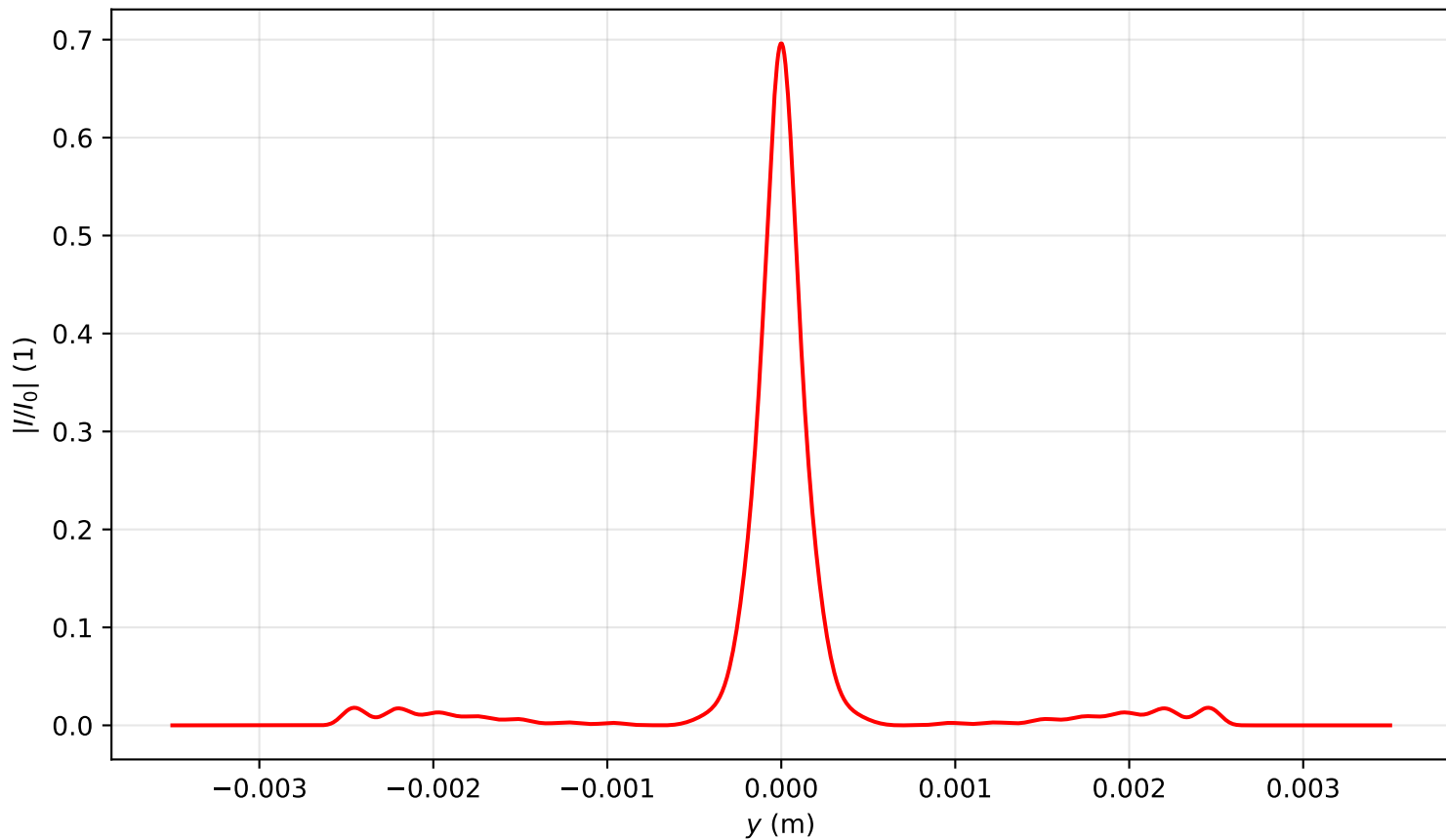
Intensity profile I(x=0, y, z=1.751)/I_0 , \text{Pin}=7.0\text{Pcr} , artificial time
